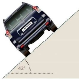
Bank Angle
